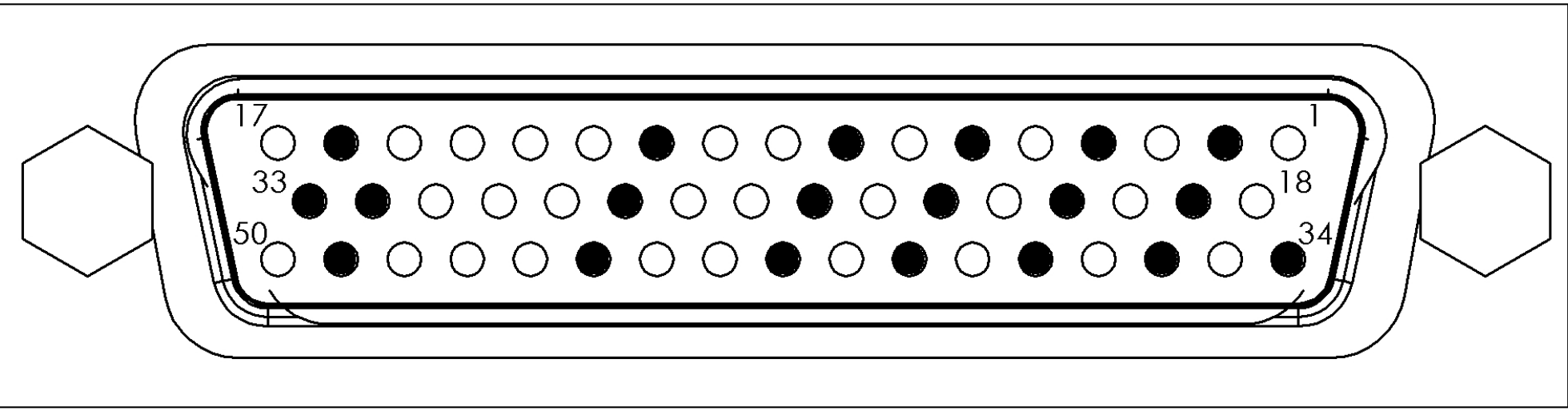
DB50 PORT: PWRBTN, DIO, PS/2, 4 x RS-232
