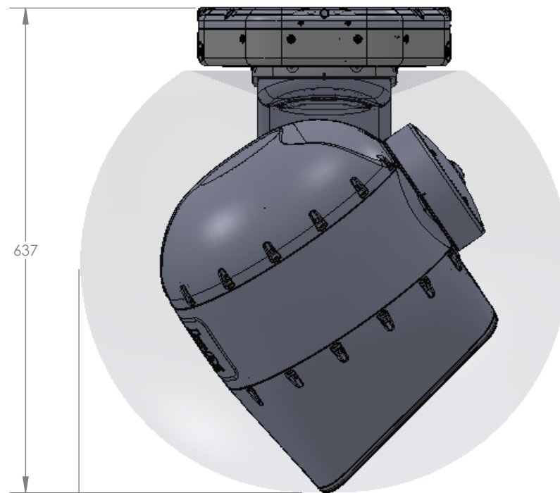
OPERATION ENVELOPE
